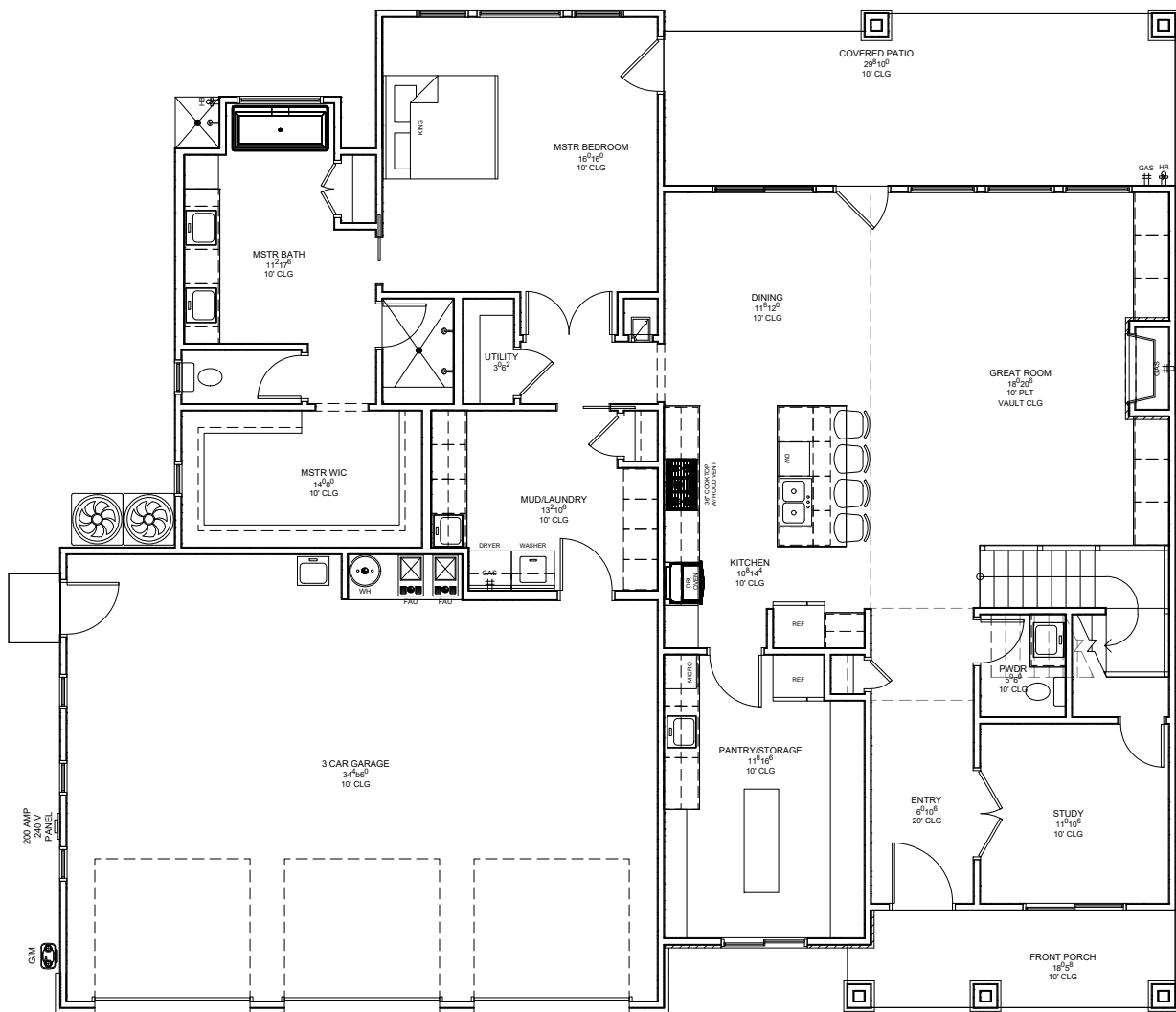
MAIN FLOOR
