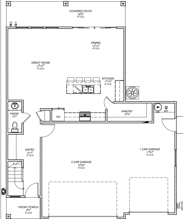
MAIN FLOOR
