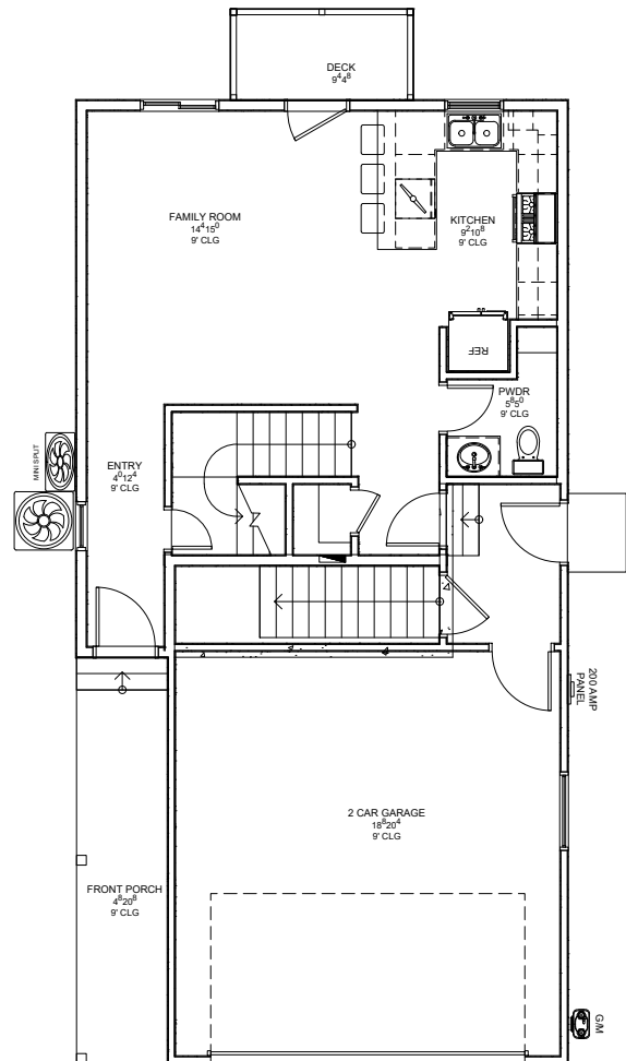
MAIN FLOOR
