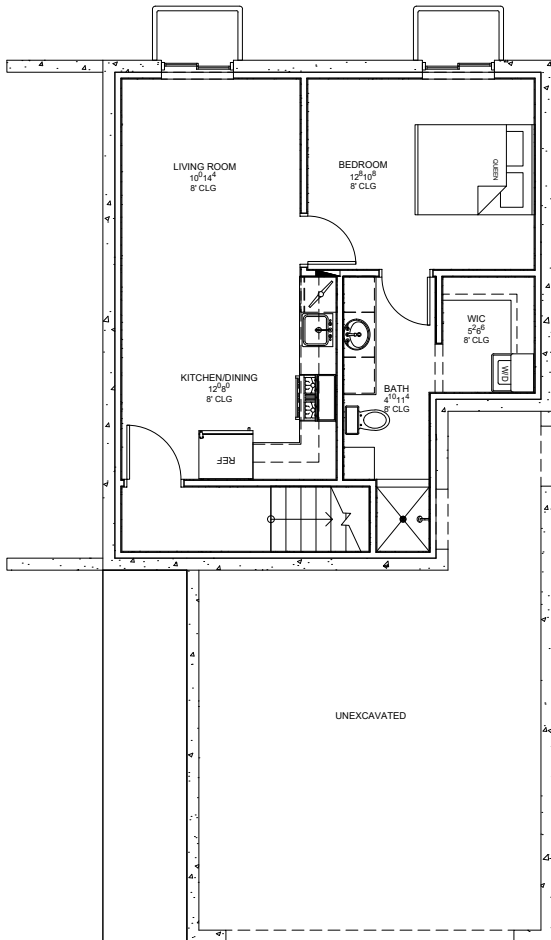
BASEMENT FLOOR
