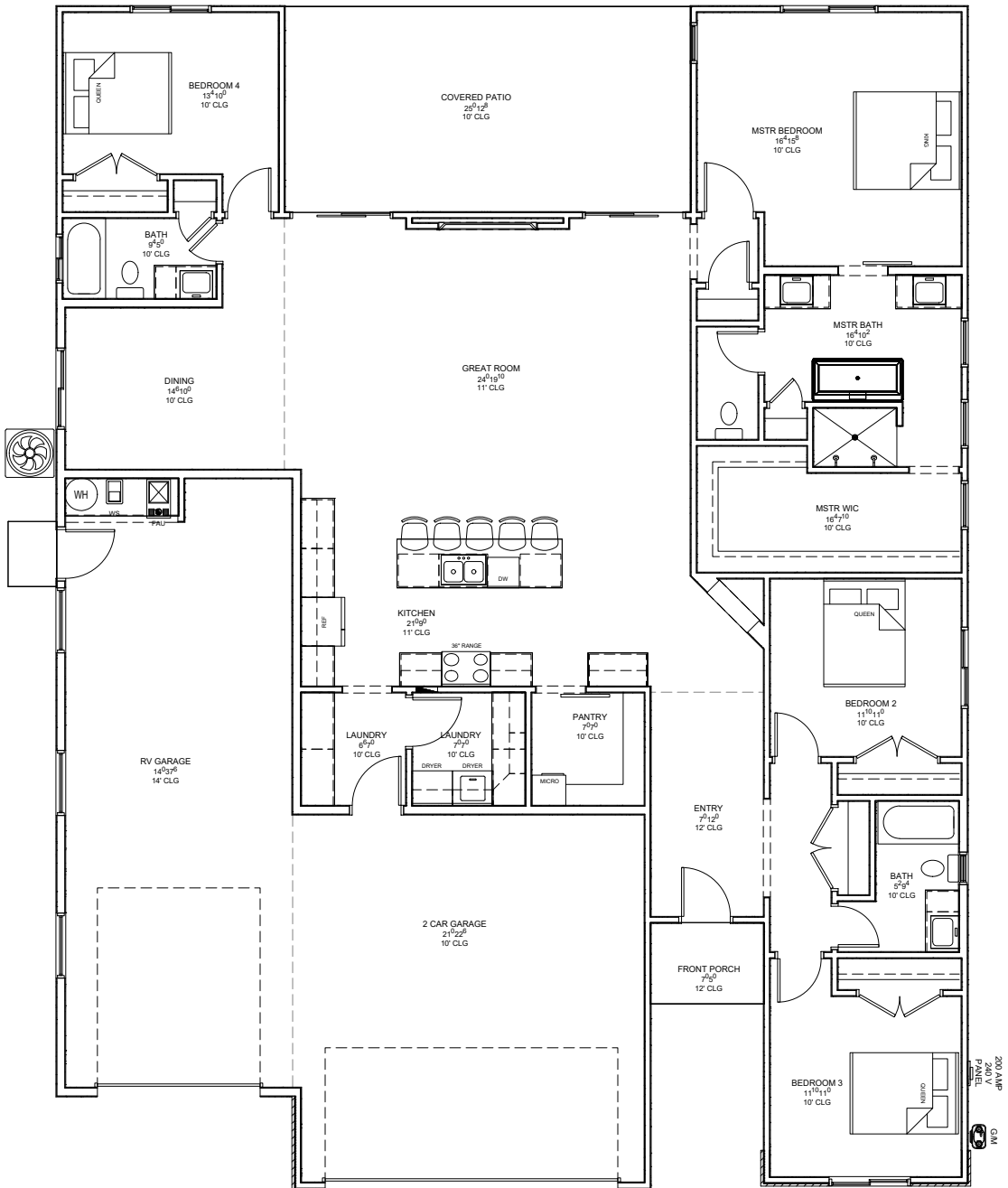
MAIN FLOOR
