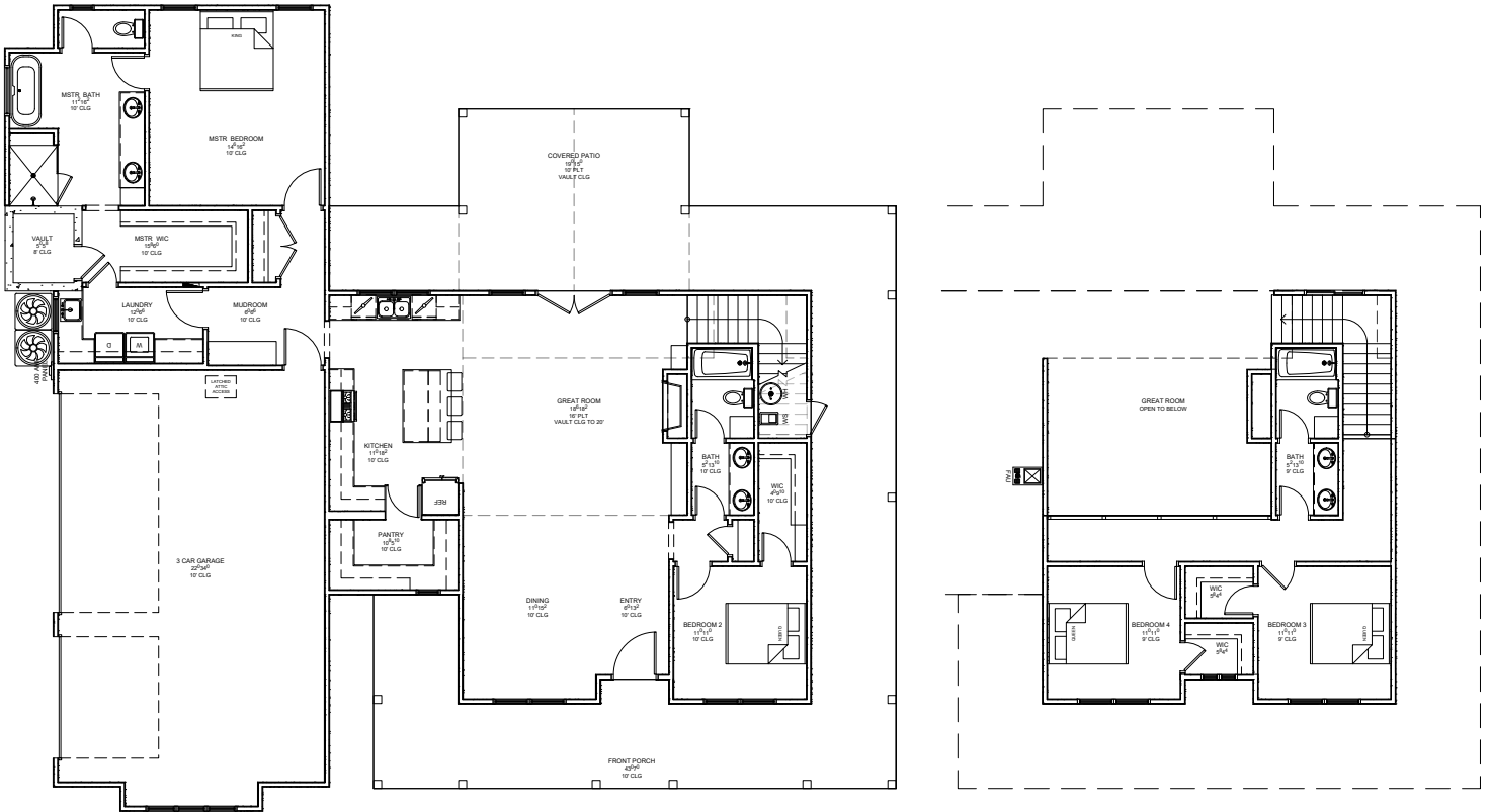
MAIN FLOOR
