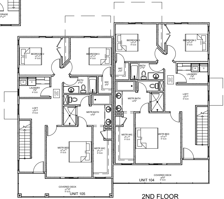
2ND FLOOR
