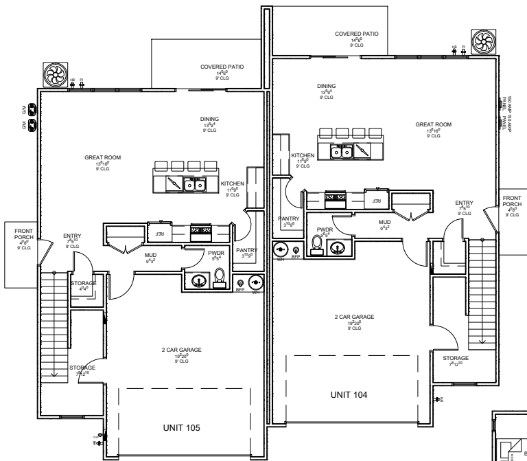
MAIN FLOOR
