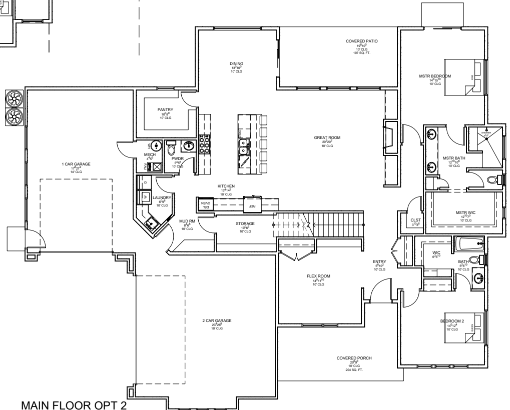
MAIN FLOOR OPT 2
