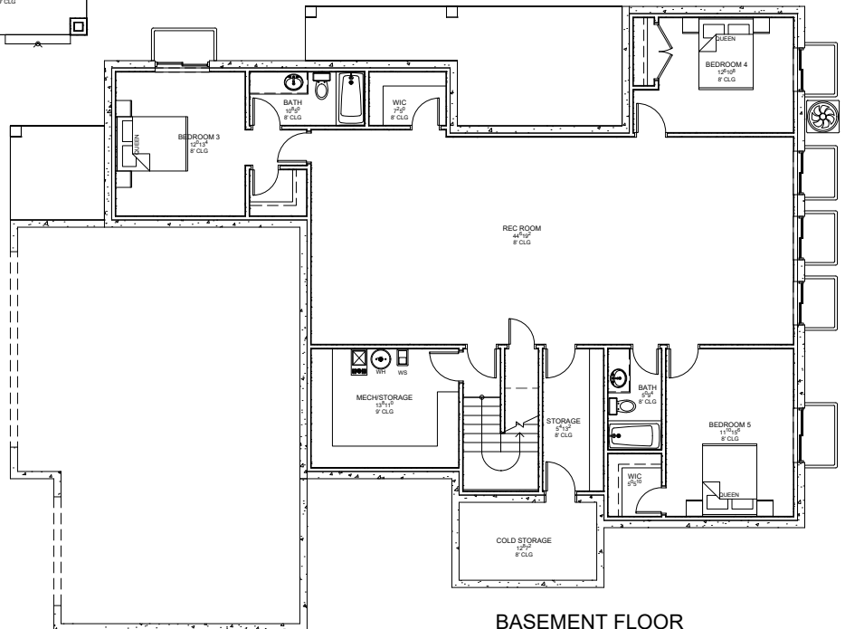
BASEMENT FLOOR
