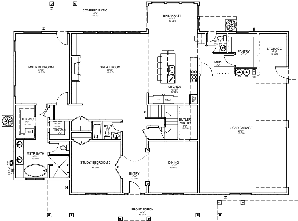
MAIN FLOOR
