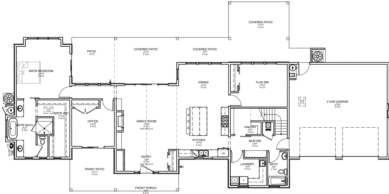
MAIN FLOOR
