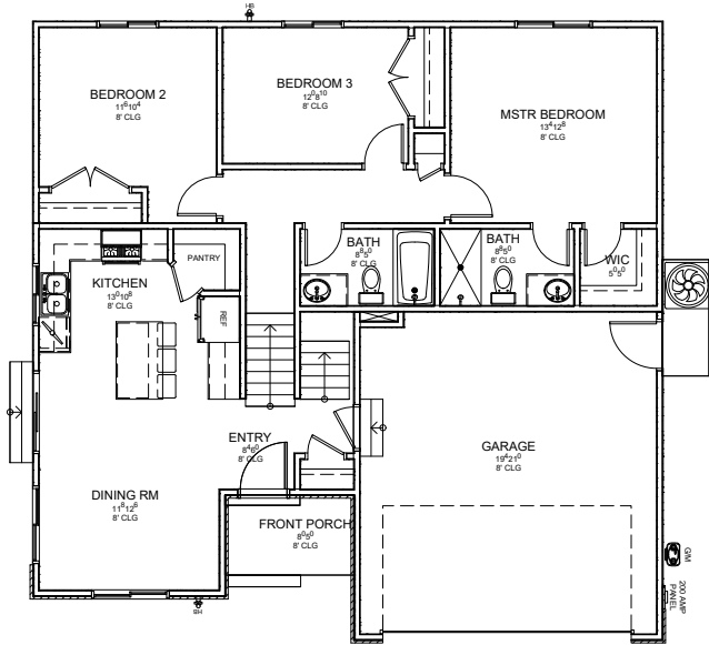
MAIN FLOOR OPT. 1
