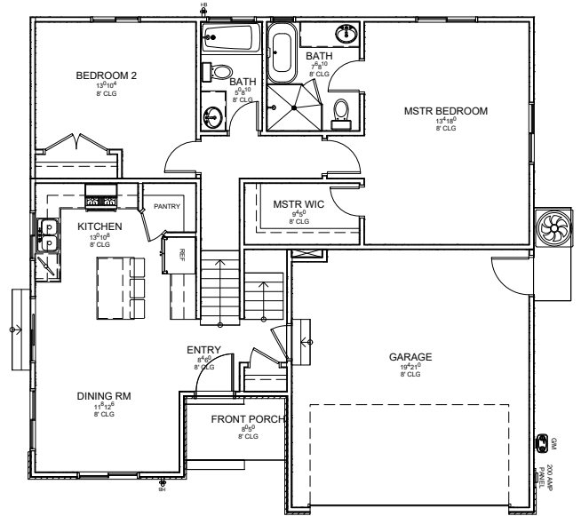
MAIN FLOOR OPT. 2
