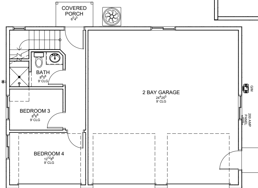
MAIN FLOOR
