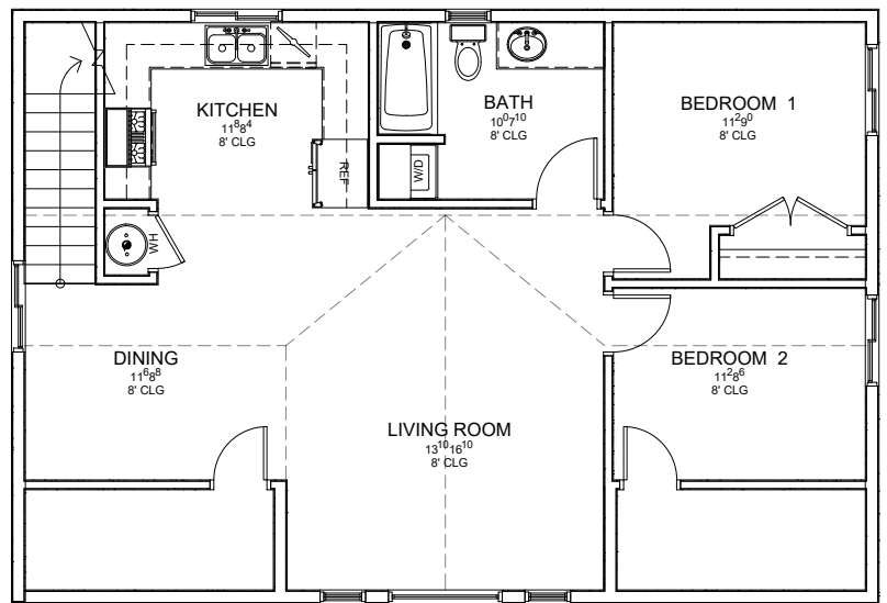
2ND FLOOR
