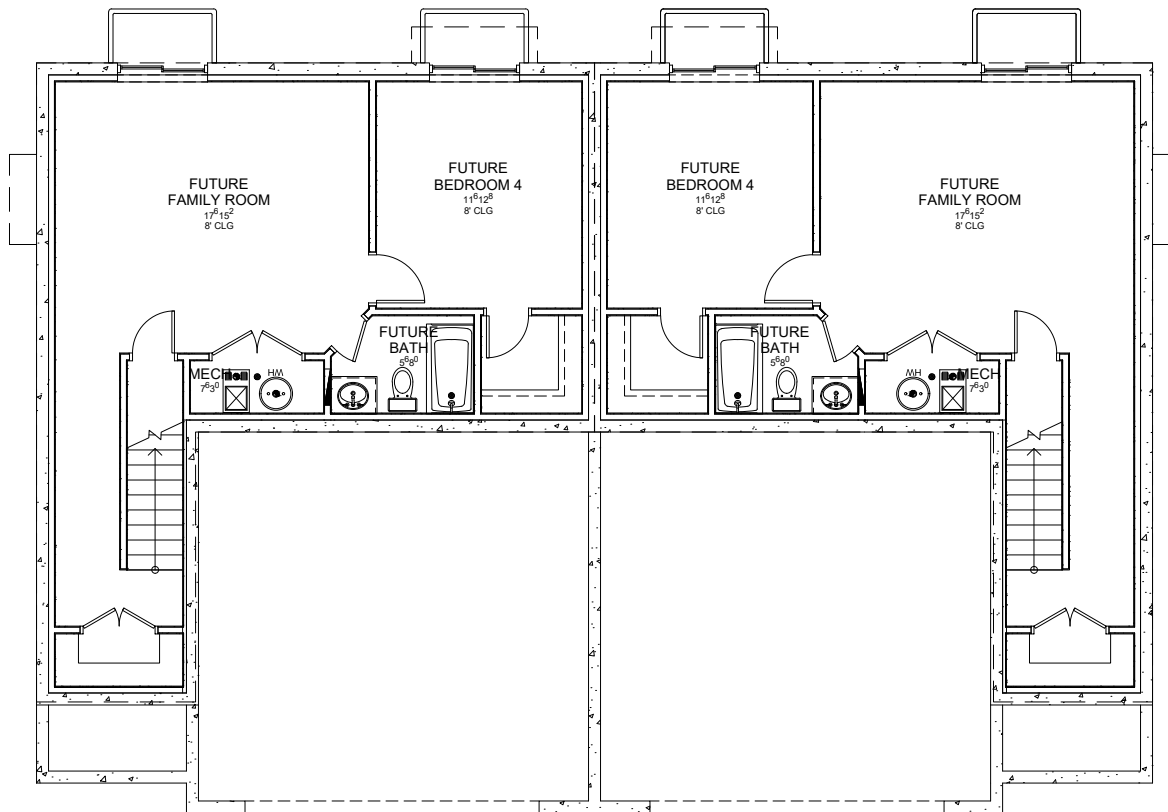
BASEMENT FLOOR
