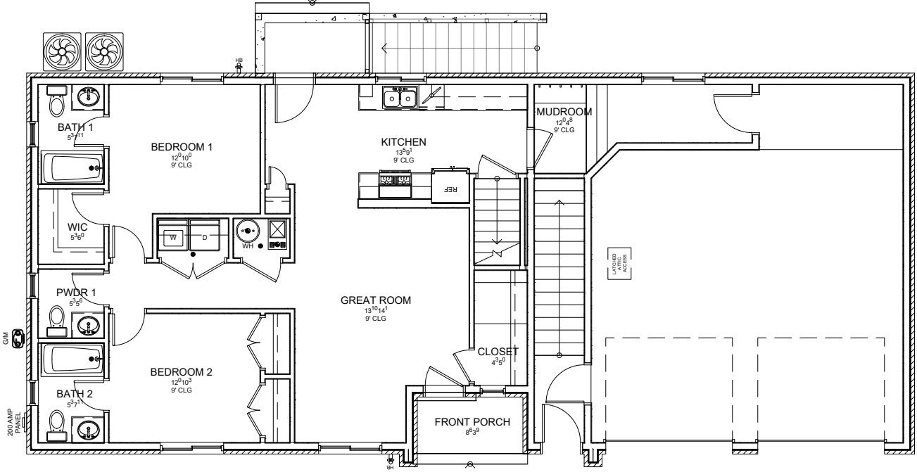
MAIN FLOOR
