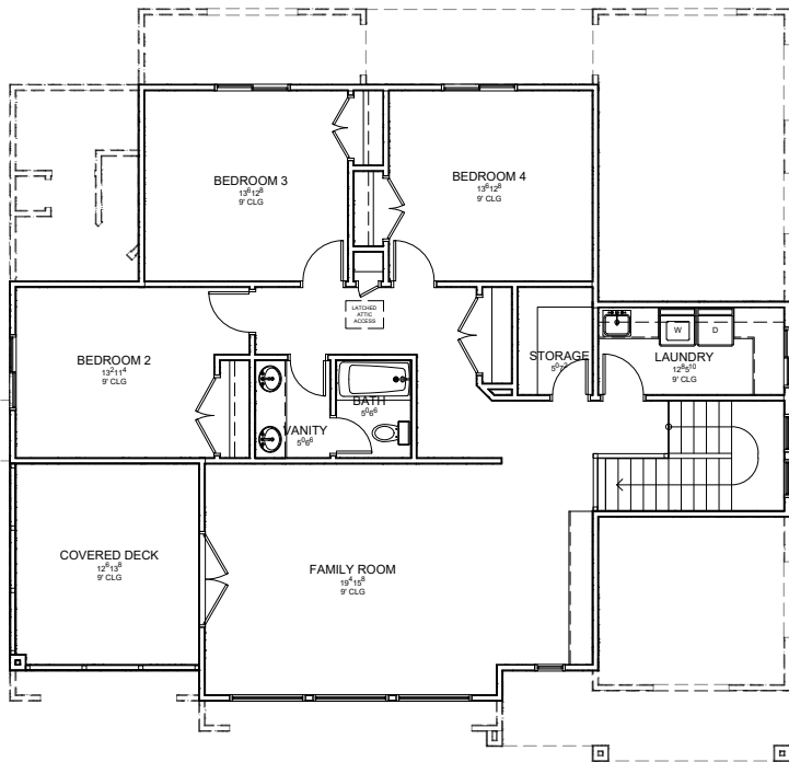
2ND FLOOR
