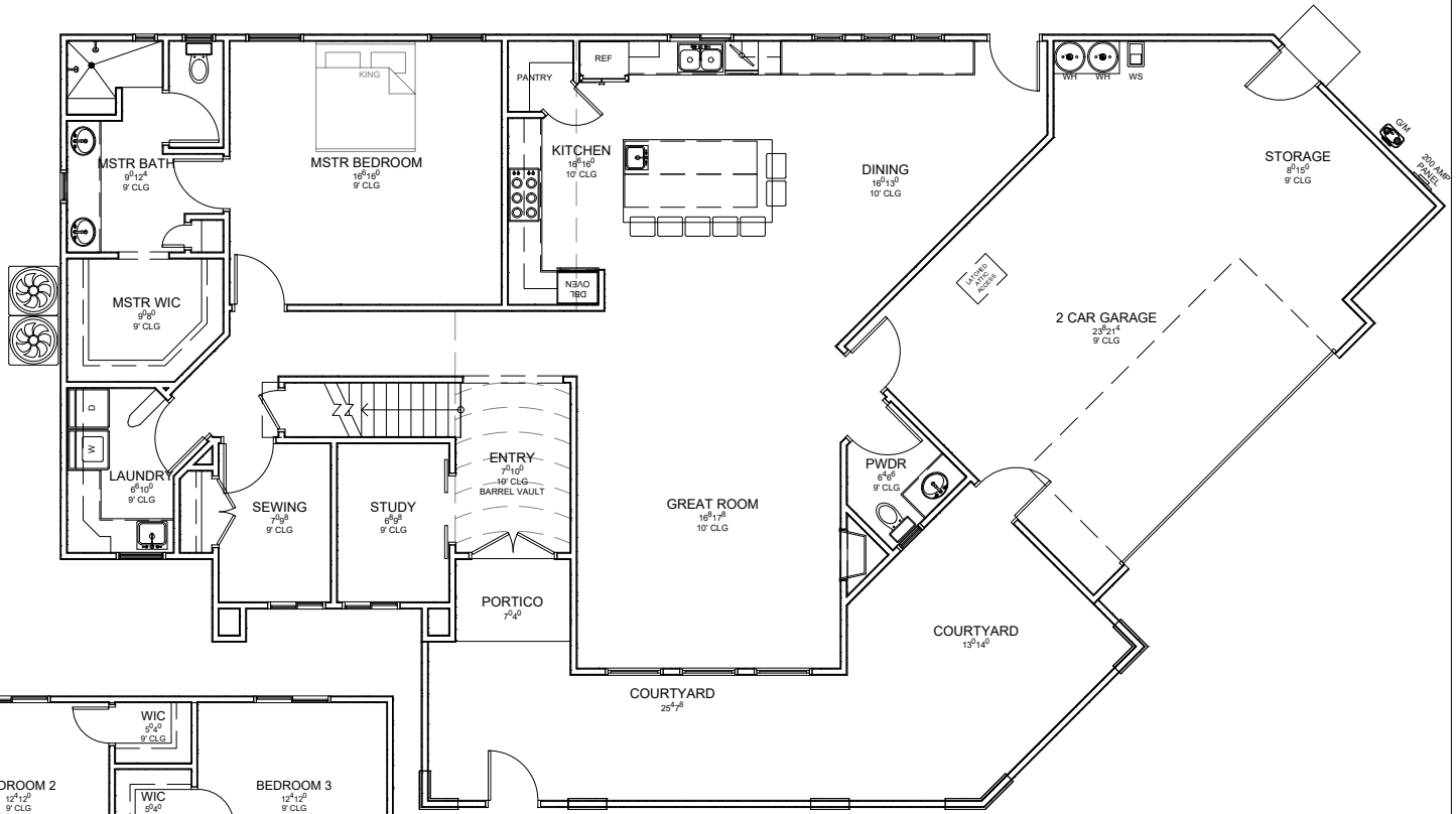
MAIN FLOOR
