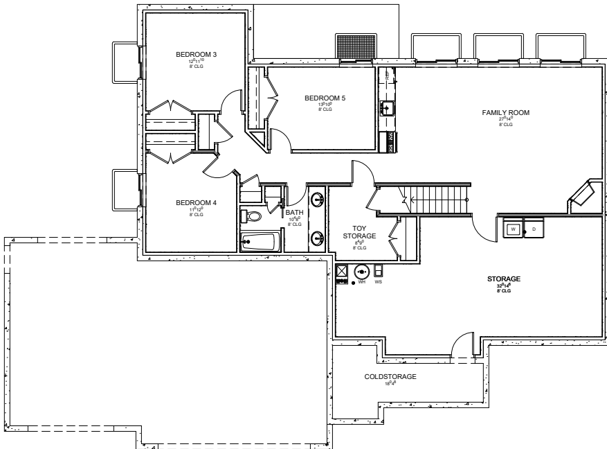
BASEMENT FLOOR
