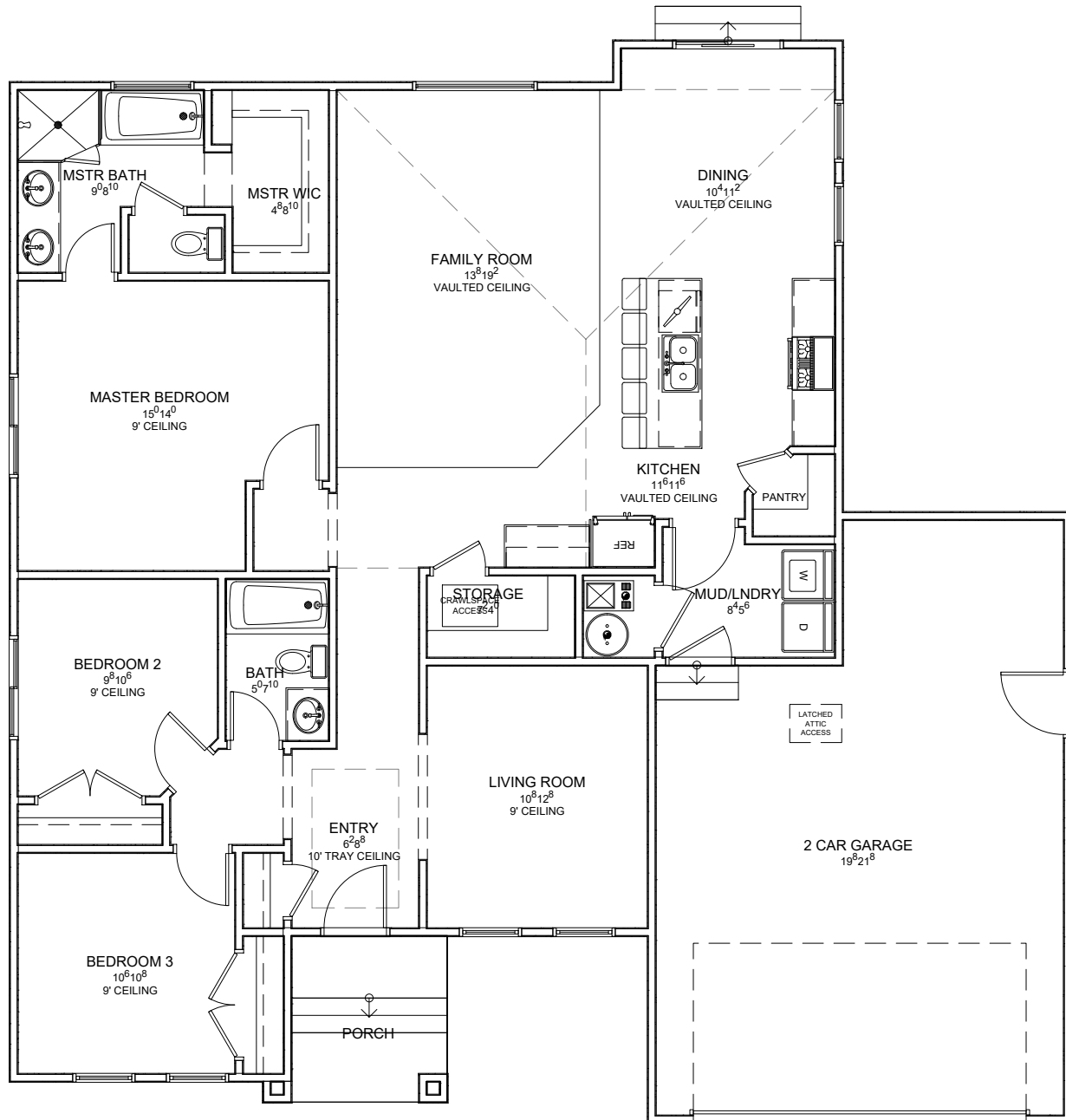
MAIN FLOOR
