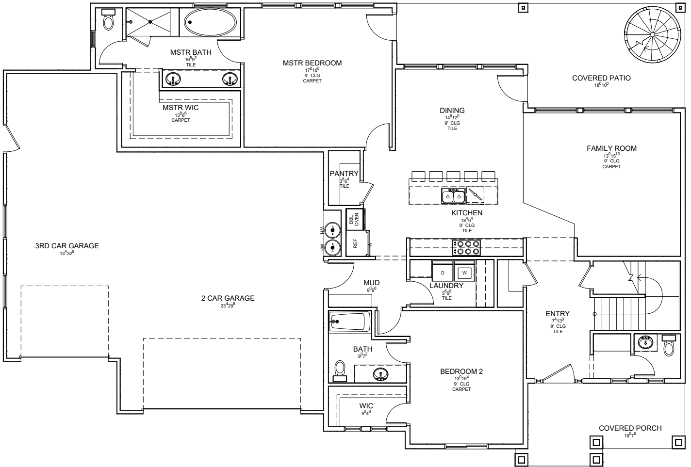
MAIN FLOOR
