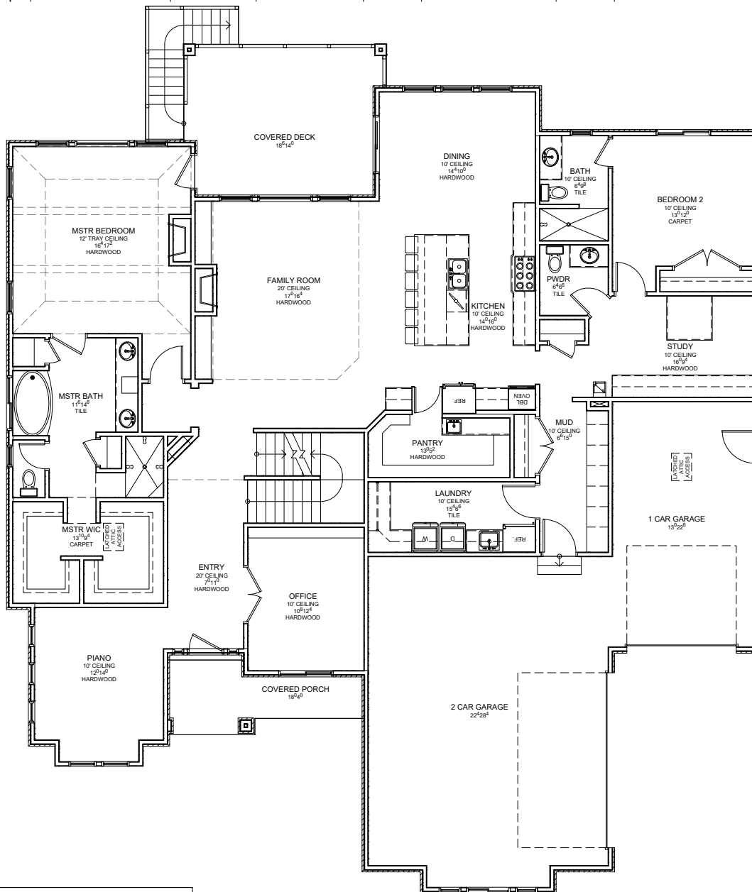
MAIN FLOOR
