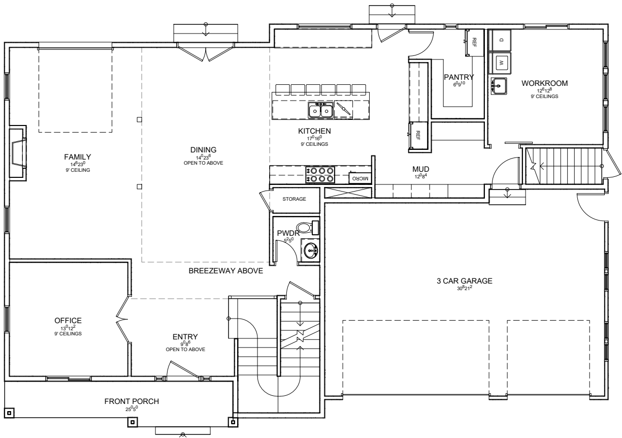
MAIN FLOOR
