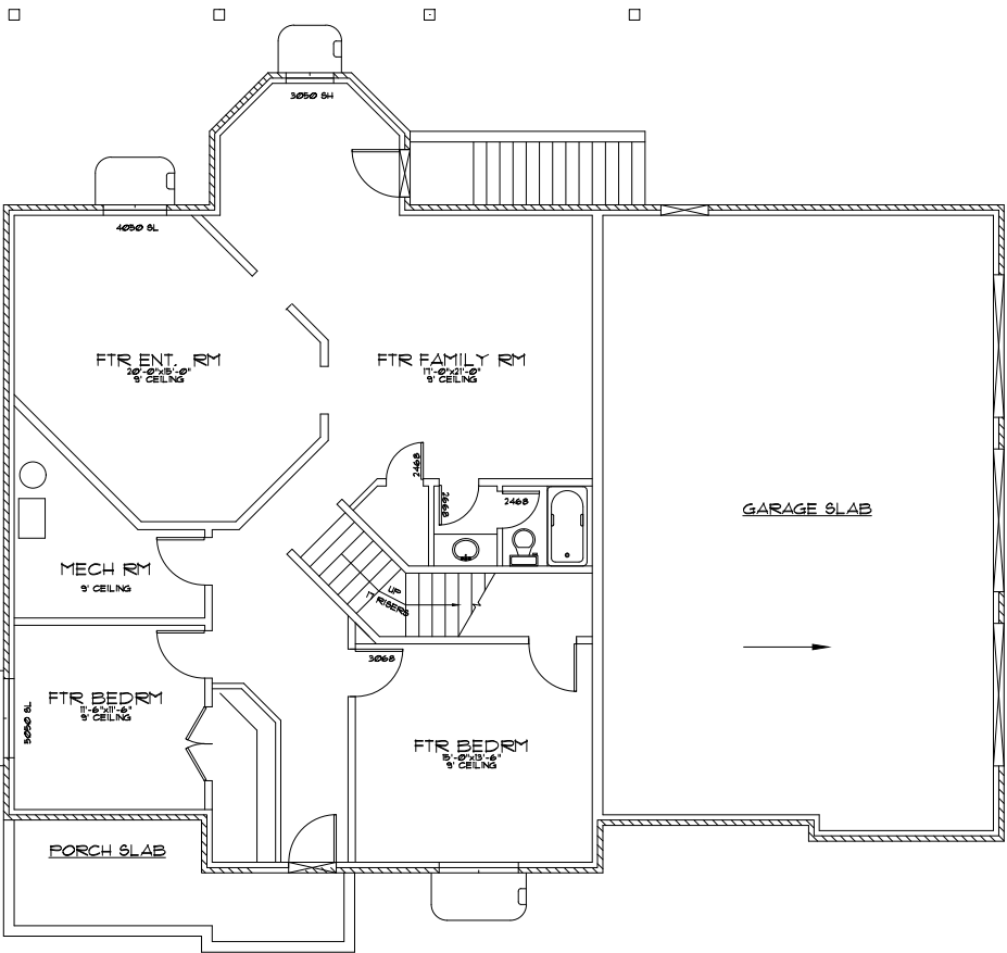
BASEMENT FLOOR
