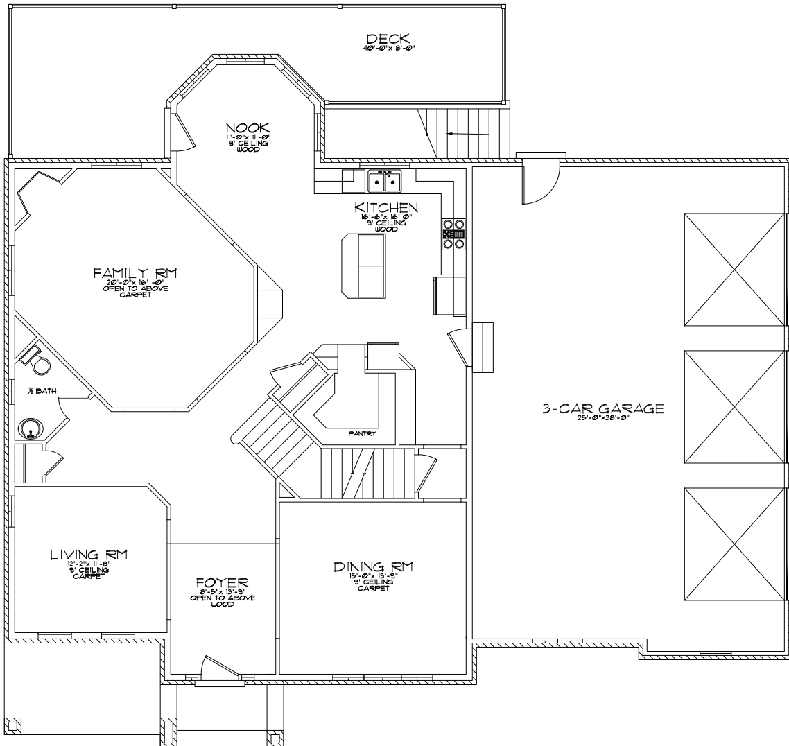
MAIN FLOOR
