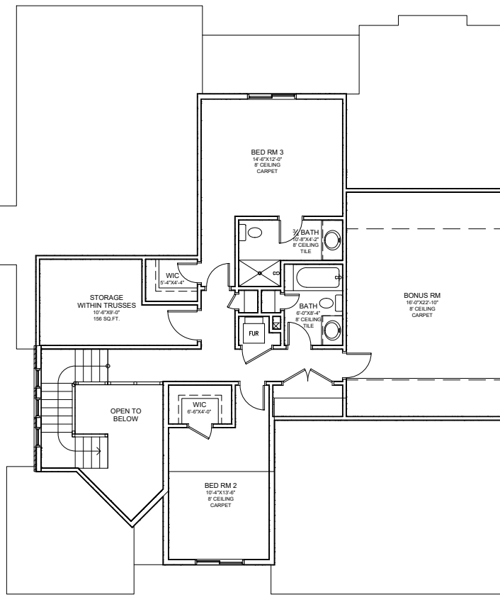
2ND FLOOR
