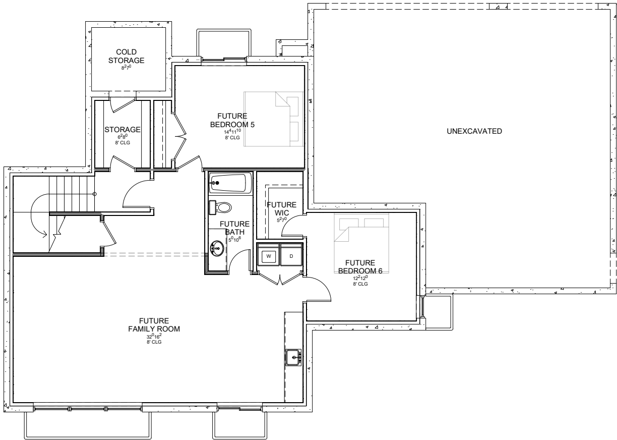
BASEMENT FLOOR
