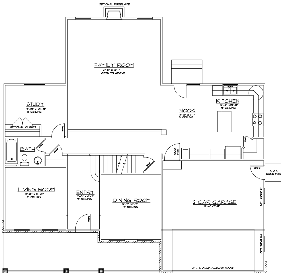
MAIN FLOOR
