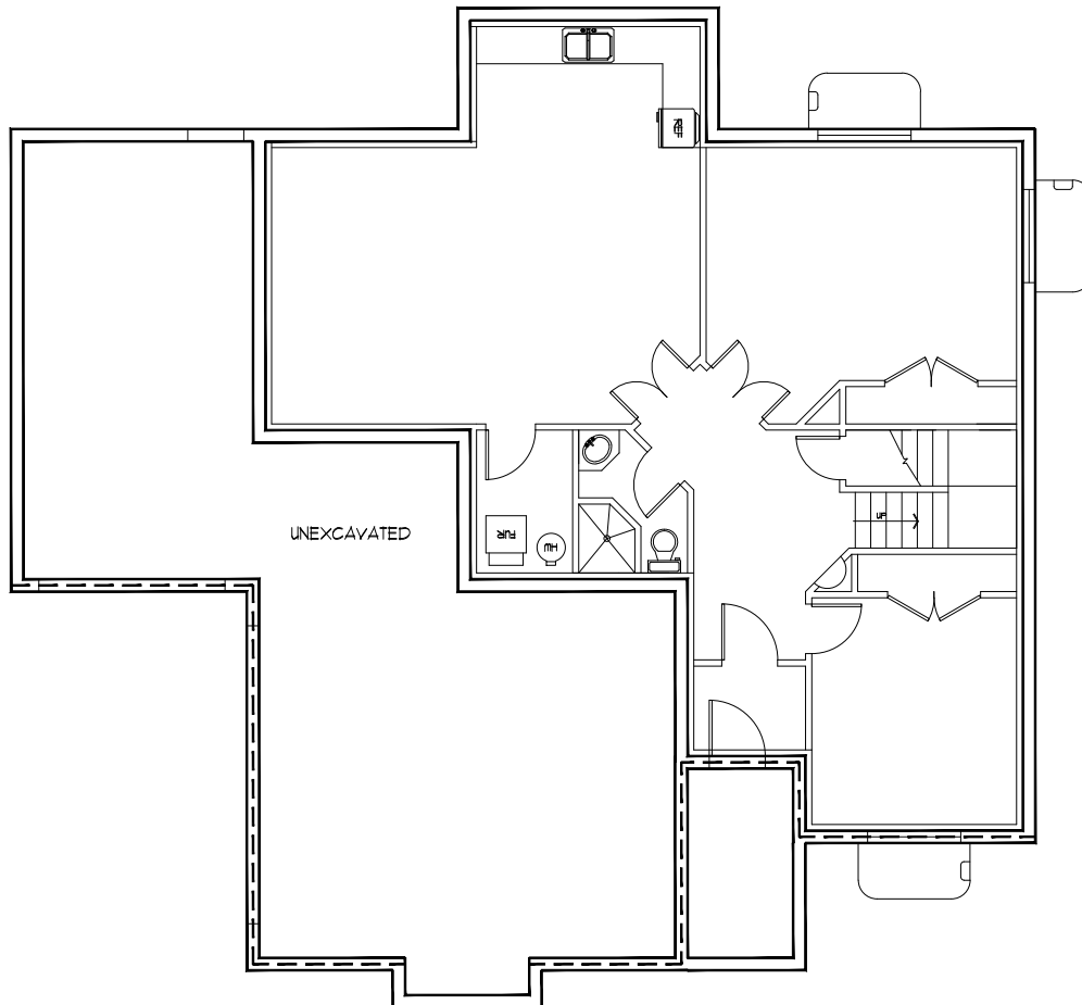
BASEMENT FLOOR
