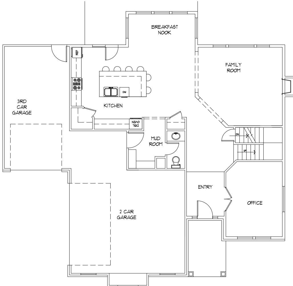
MAIN FLOOR
