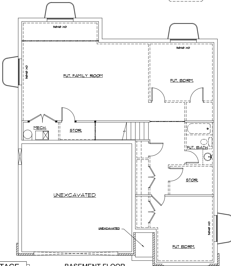
BASEMENT FLOOR
