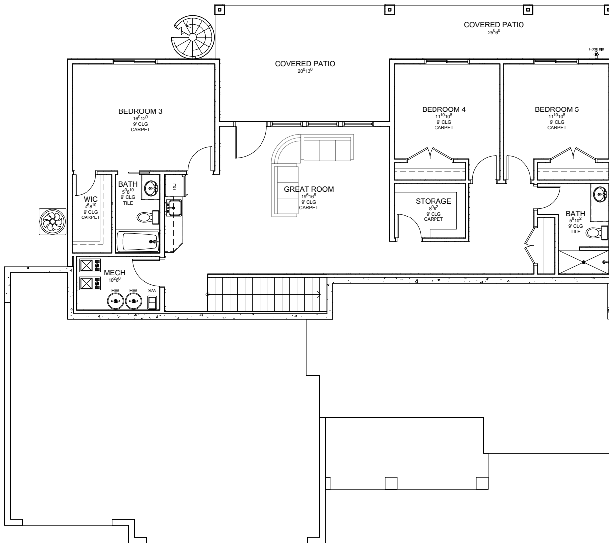
BASEMENT FLOOR OPTION 1
