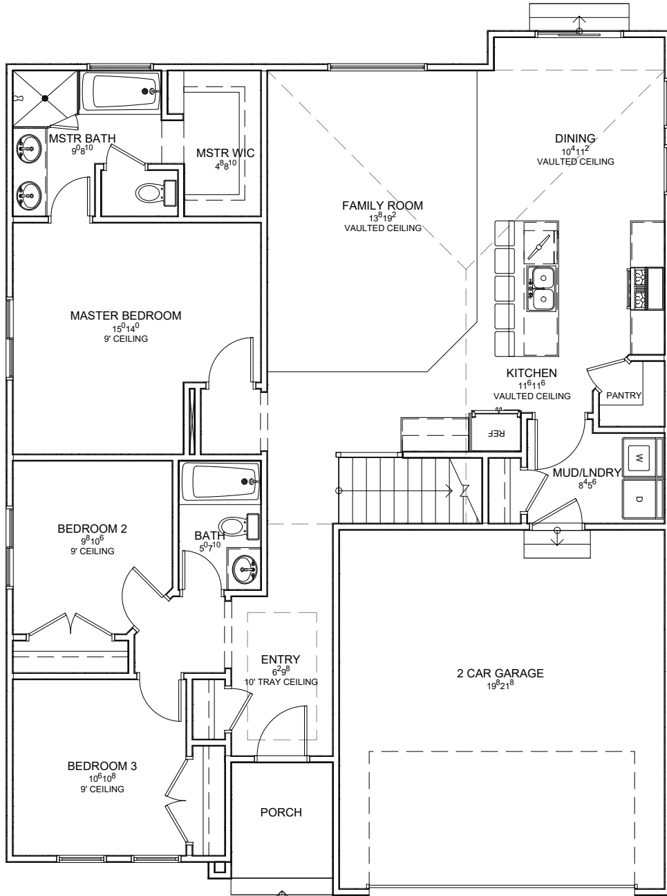
MAIN FLOOR
