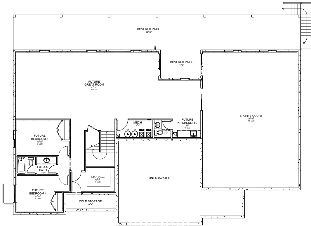
BASEMENT FLOOR OPTION 2
