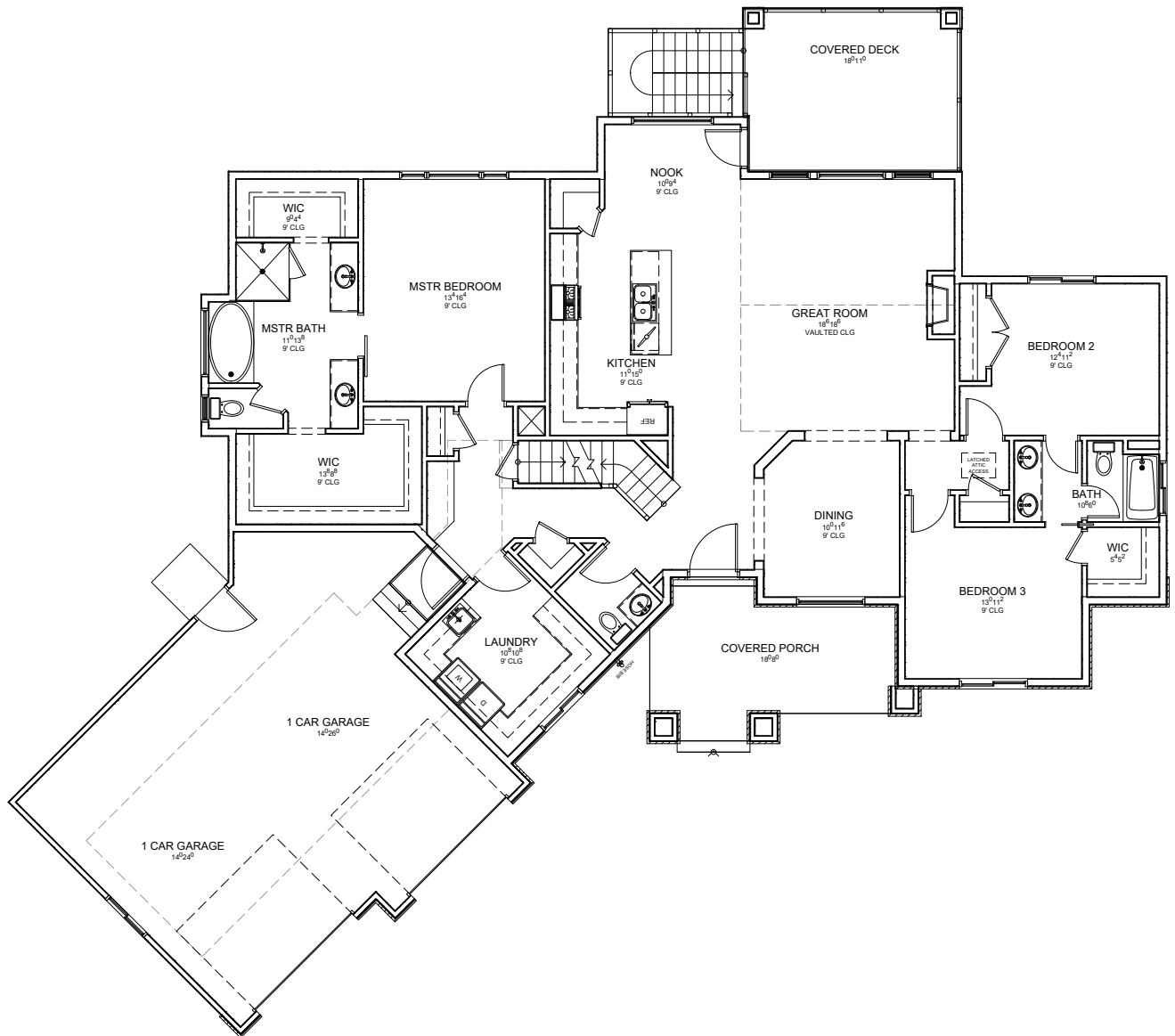
MAIN FLOOR
