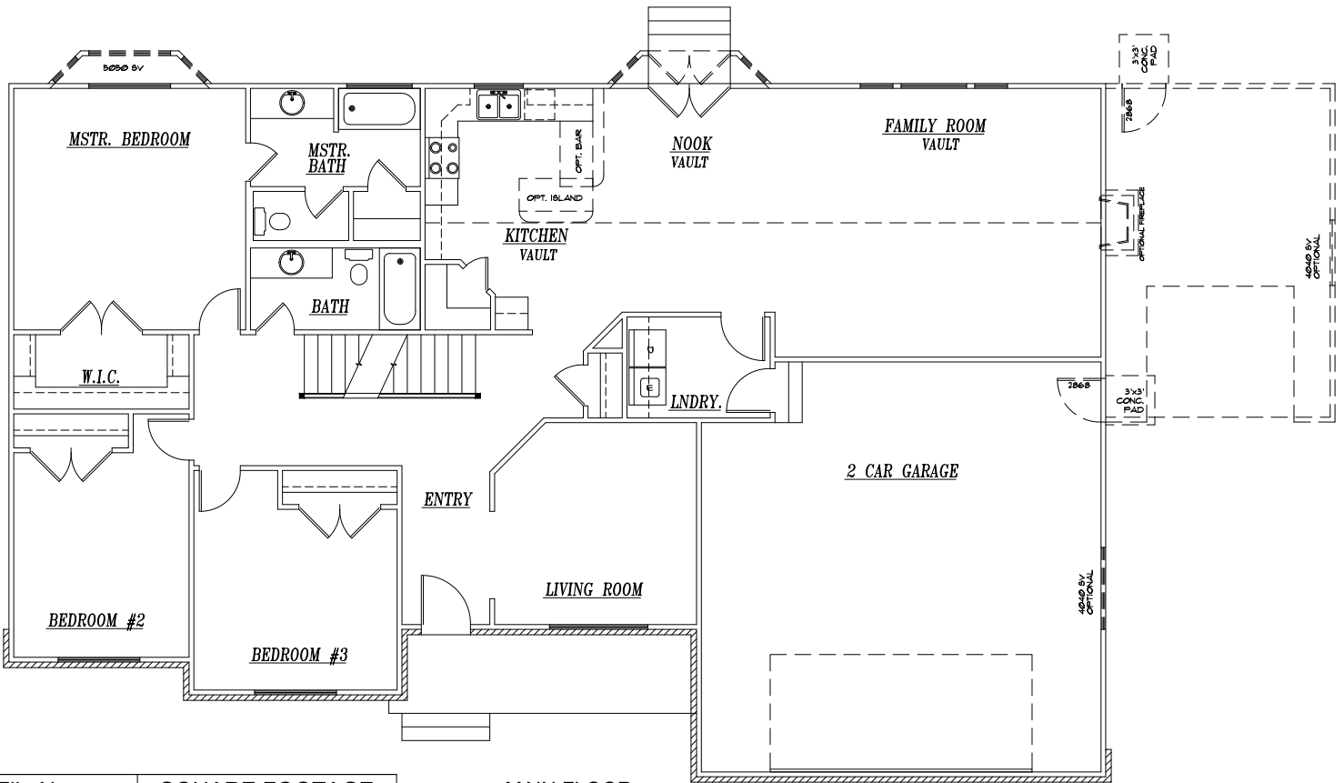
MAIN FLOOR
