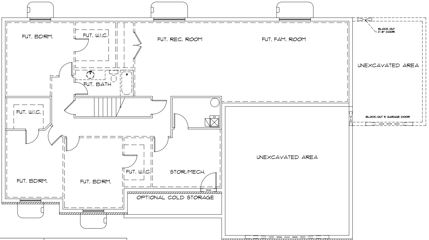
BASEMENT FLOOR
