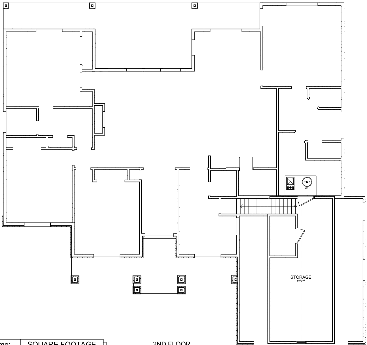
2ND FLOOR
