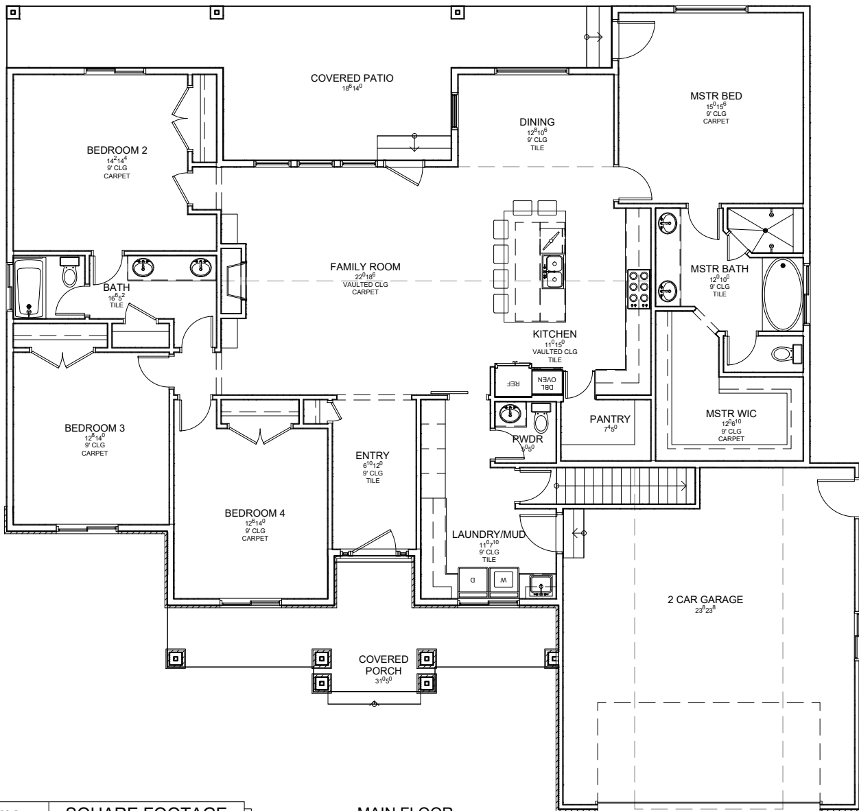
MAIN FLOOR
