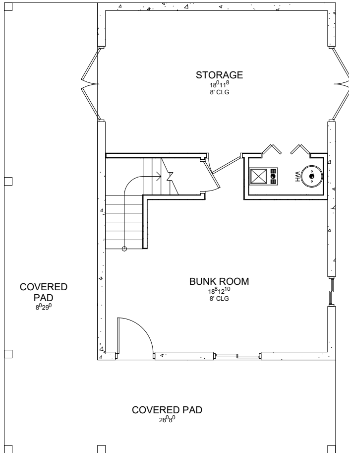
BASEMENT FLOOR
