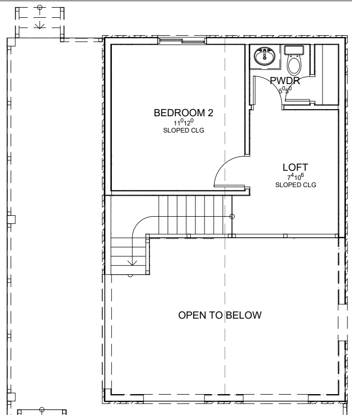
UPPER FLOOR
