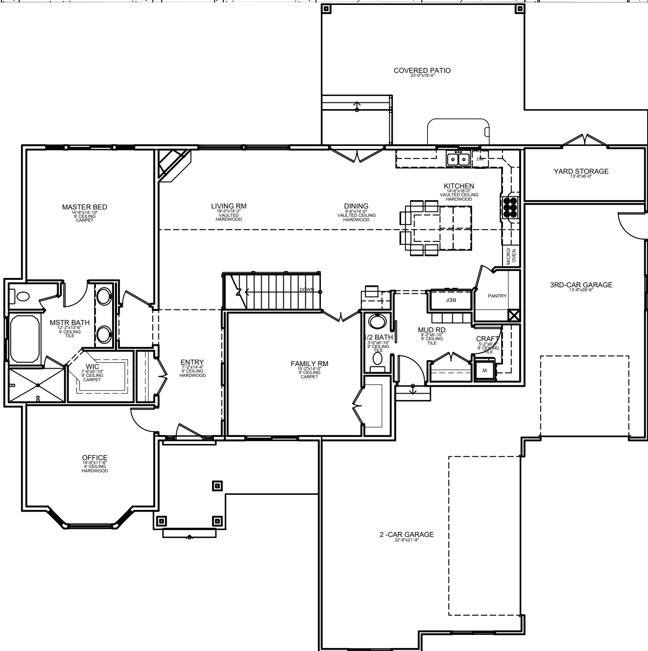
MAIN FLOOR
