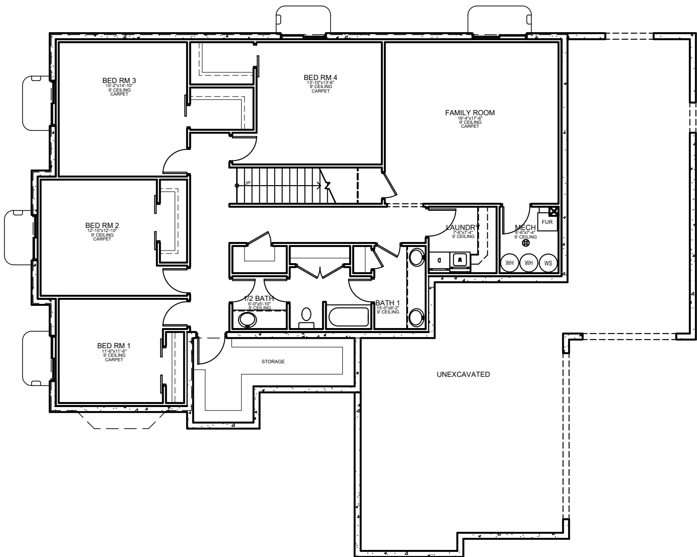
BASEMENT FLOOR
