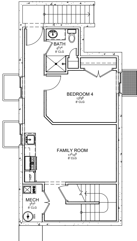
BASEMENT FLOOR
