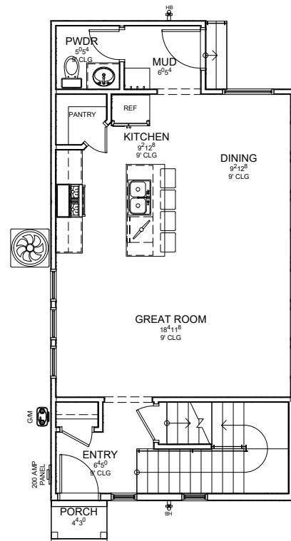
MAIN FLOOR
