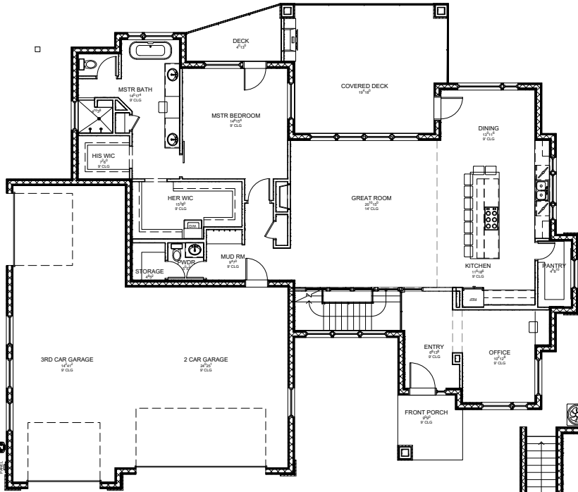
MAIN FLOOR
