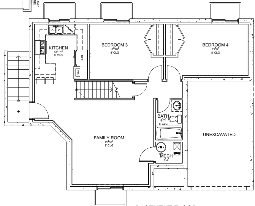
BASEMENT FLOOR
