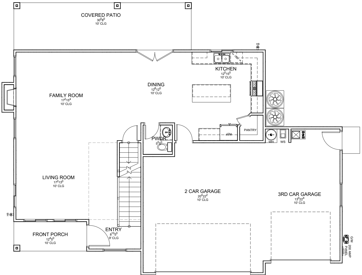
MAIN FLOOR
