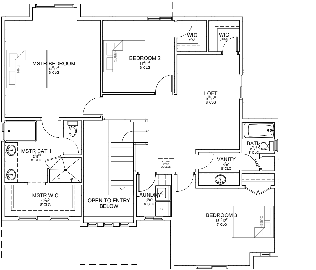
2ND FLOOR
