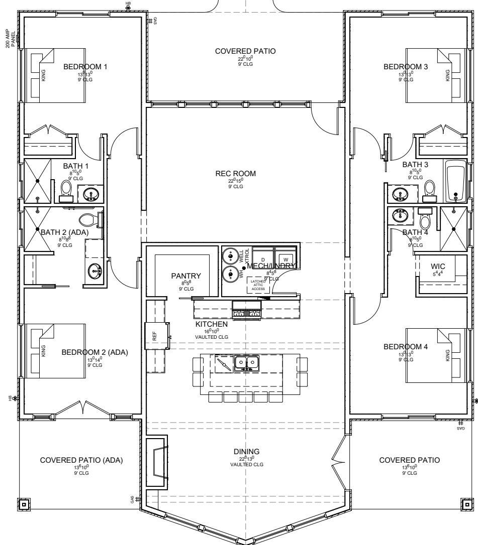
MAIN FLOOR
