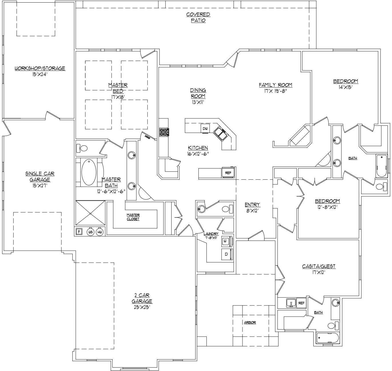
MAIN FLOOR
