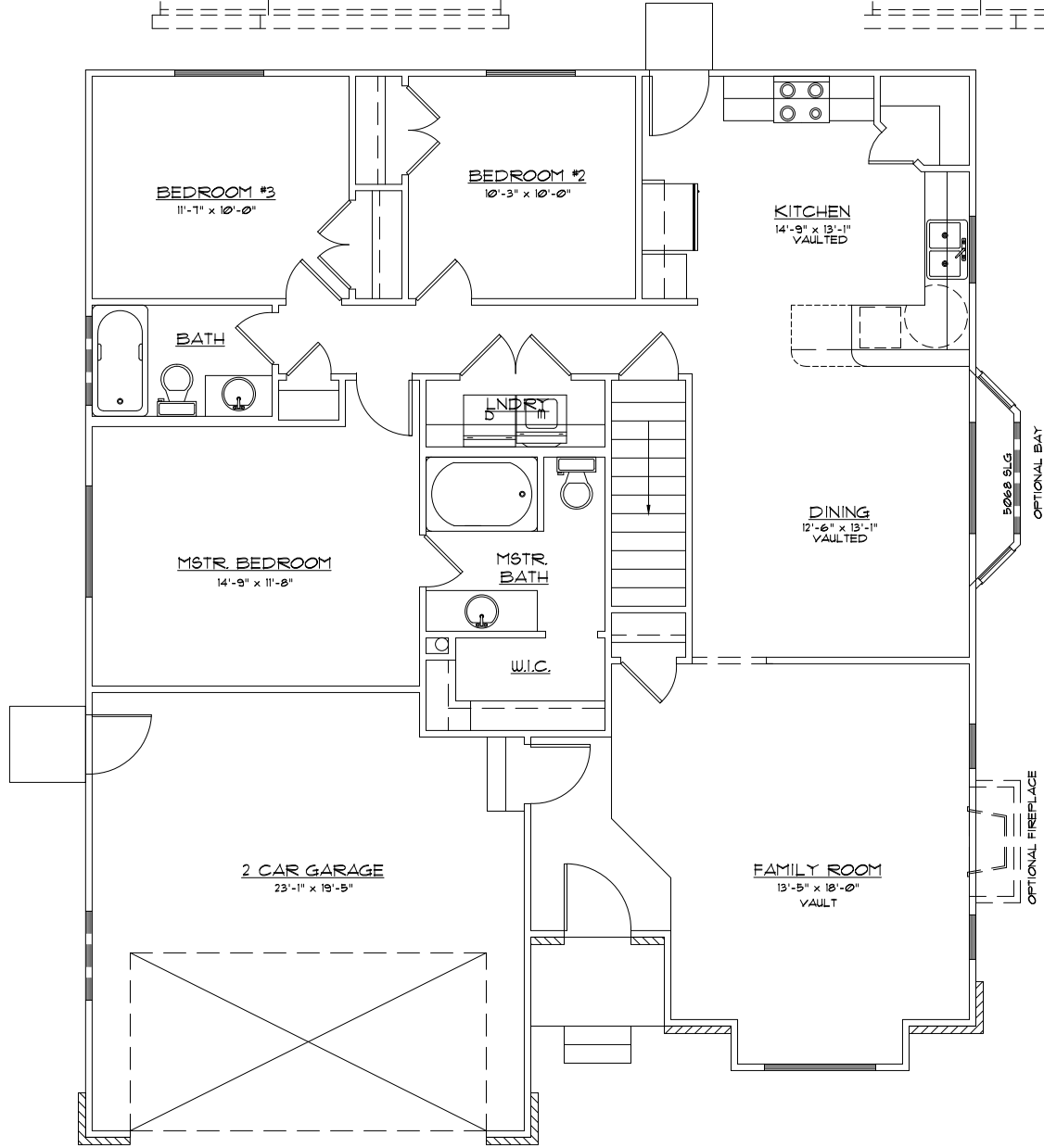
MAIN FLOOR
